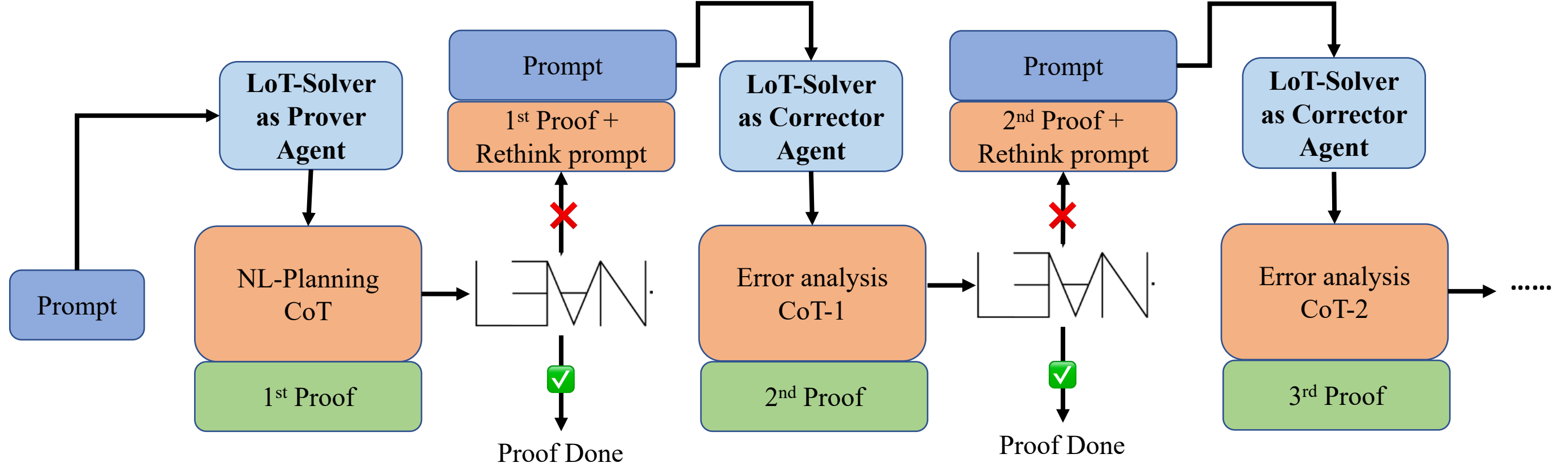
(a) Multi-Agent Lean-based Long CoT inference
