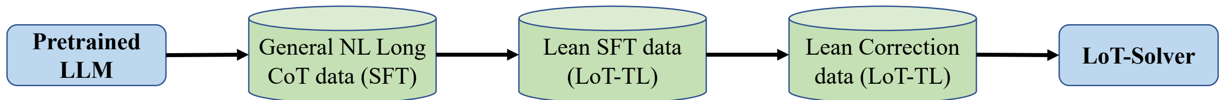
(c) Training procedure of LoT-Solver
