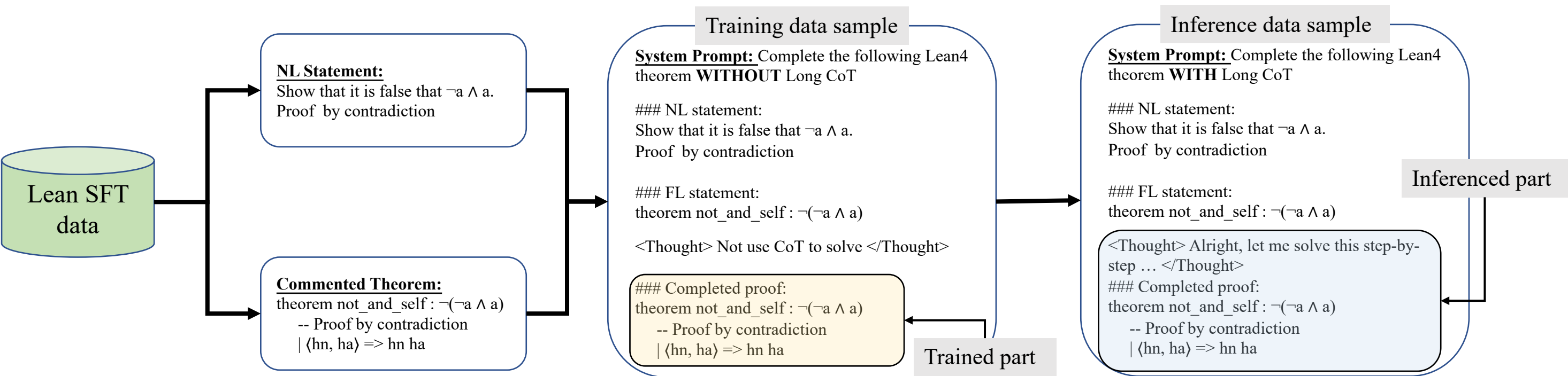
(b) LoT-TL Training-Inference pipeline
