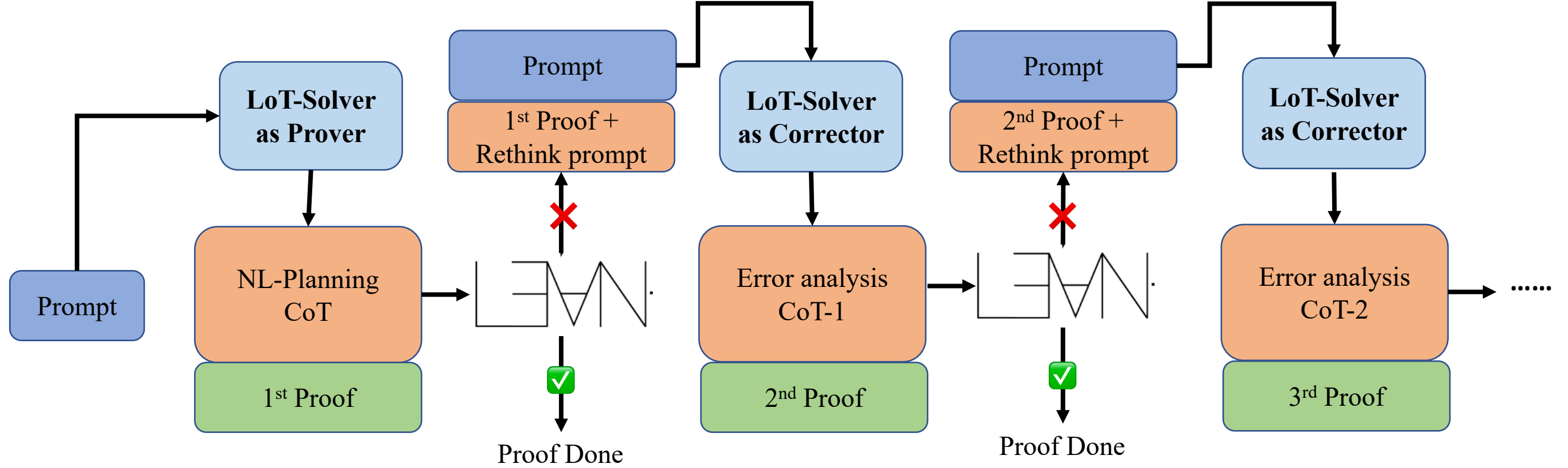
(a) Model-Collaboration Lean-based Long CoT inference
